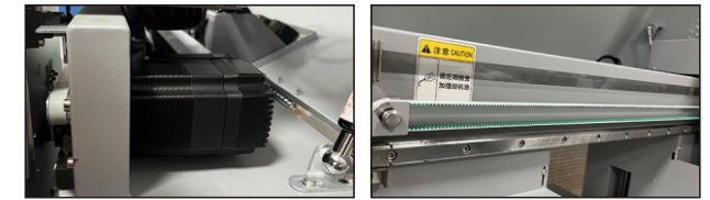
Servo motor, Leadshine motor Import the Taiwan SHAC guide rail
